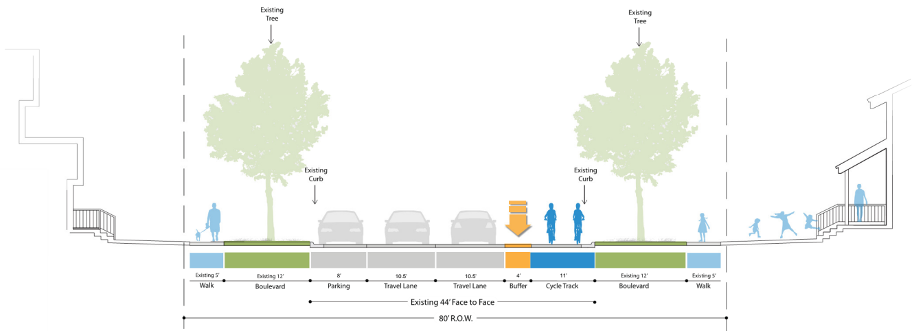
PRAIRIE STREET ON-STREET CYCLE TRACK
