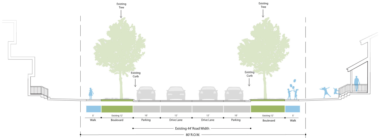
PRAIRIE STREET EXISTING
